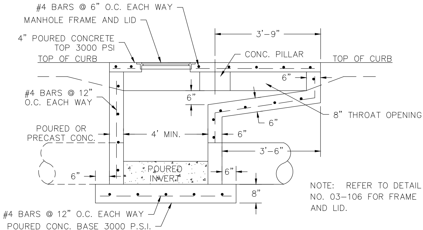
SECTION X-X
